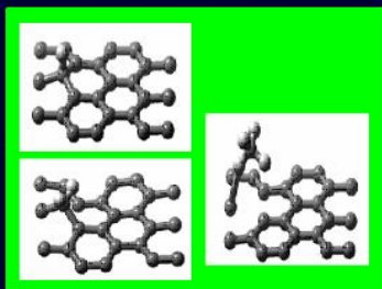
Methan production on graphite
