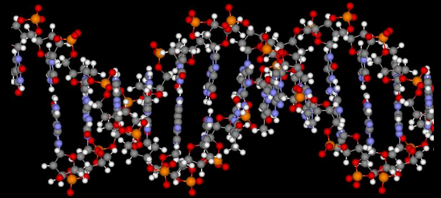
Double-stranded DNA
