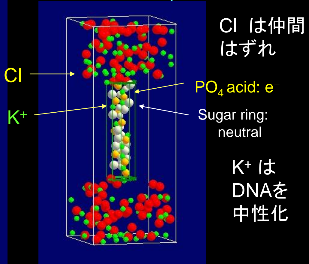
DNA-stuffed pore
