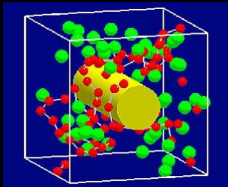
Charge inversion
