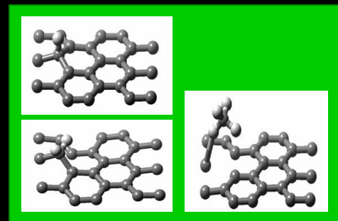
Graphene destruction by hydrogen adsorption
