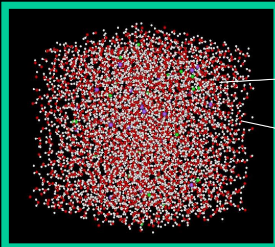
Waters with hydrogen bond H--O
