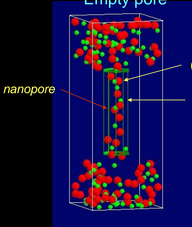
Empty pore
