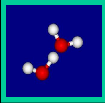
Waters with hydrogen bond H--O
